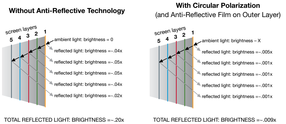
Figure 1. The reduction of reflected light enabled by circular polarization
