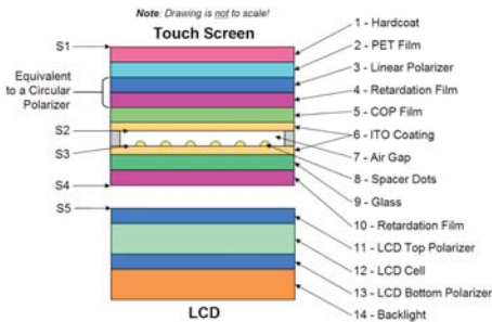
Figure 3: The application of a circular polarizer to a resistive touch screen.
